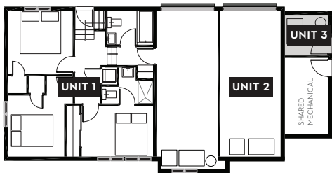
FLOORPLATE LEVEL 1
